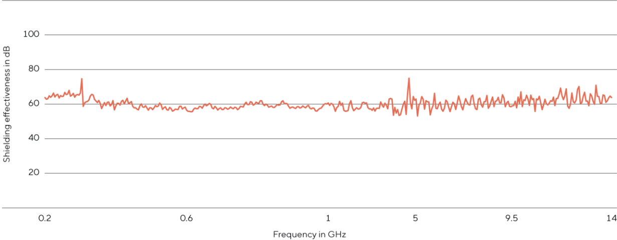
Shielding effectiveness 0.2 - 14 GHz according to IEEE 299/200
