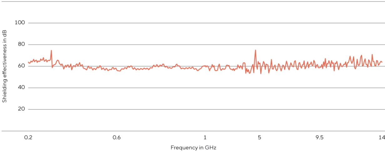
Shielding effectiveness 0.2 - 14 GHz according to IEEE 299/200
